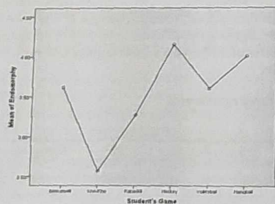
Figure 1: Mean plot of Endomorphic component
