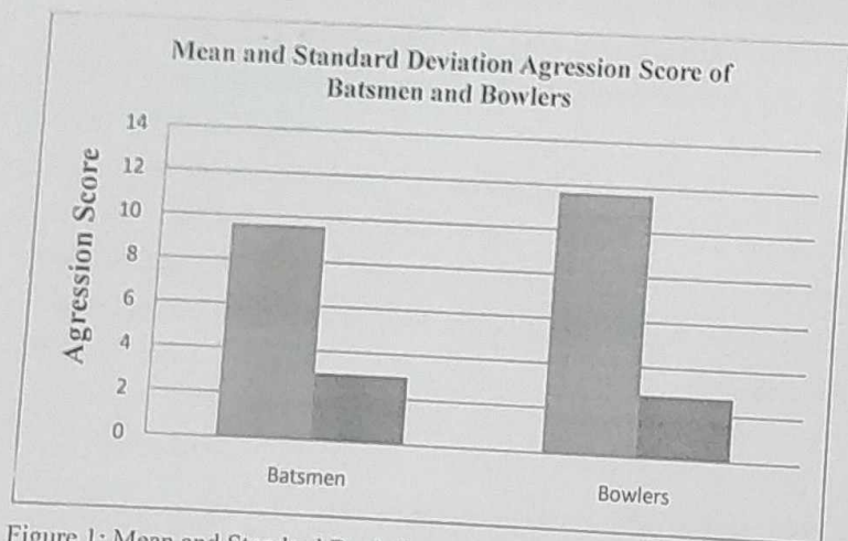
Figure 1: Mean and Standard Deviation Aggression Score of Batsmen and Bowlers
